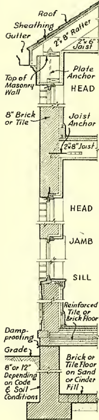
Wall Section
